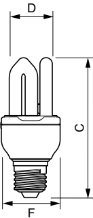
Econ Genie ErP NG 14W/865 E27 220-240V
